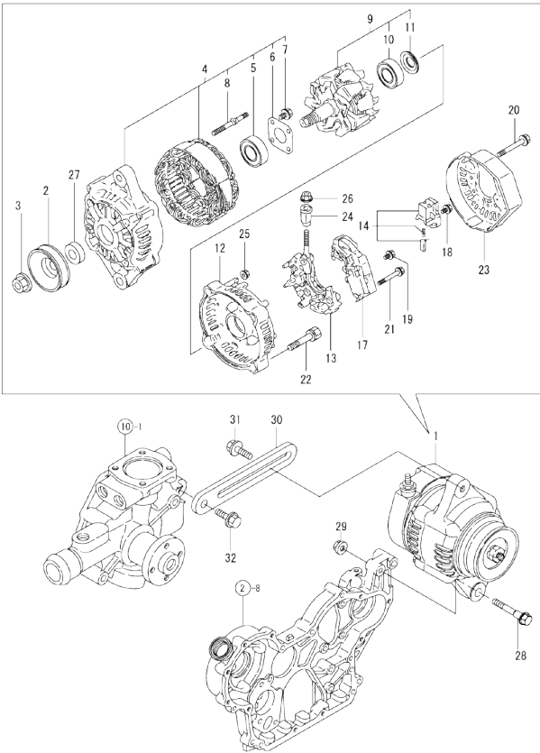
0CW10-M07700 4TNV94L-NCKMK Fig.17. (16A)GENERATOR
