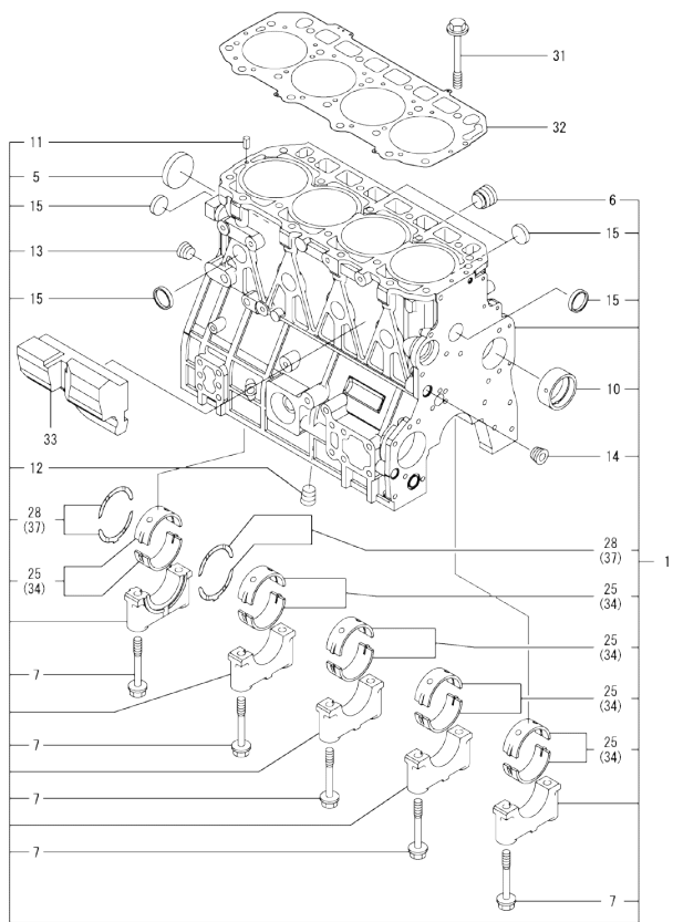
0CW10-M07700 4TNV94L-NCKMK Fig.1. CYLINDER BLOCK
