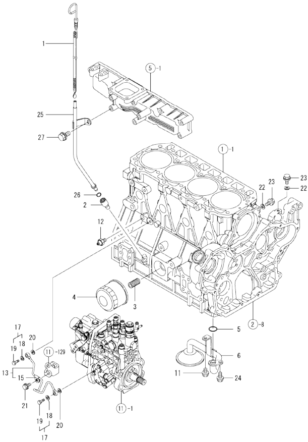
0CW10-M07700 4TNV94L-NCKMK Fig.9. LUB. OIL SYSTEM
