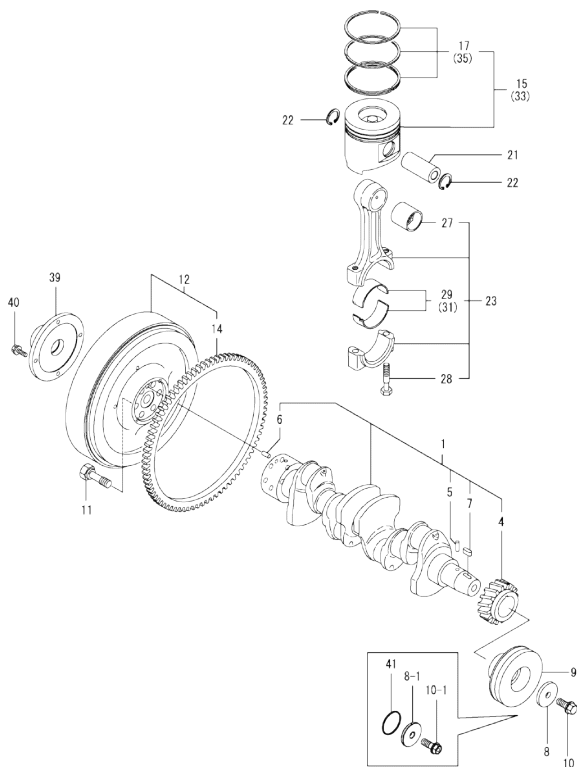
Fig.8. CRANKSHAFT & PISTON
