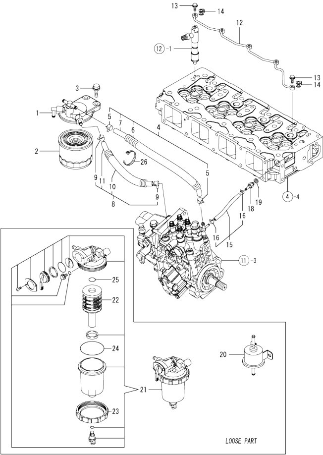
Fig.13. FUEL LINE
