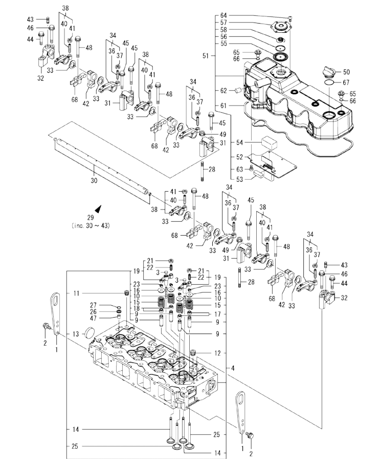
Fig.4. CYLINDER HEAD & BONNET
