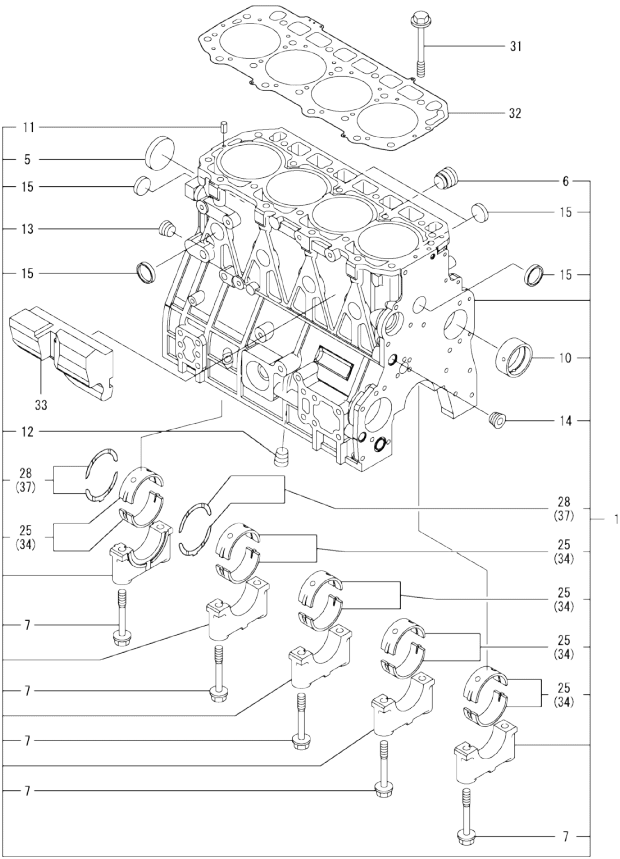
0CV10-M88900 4TNV94L-PDBWE Fig.1. CYLINDER BLOCK
