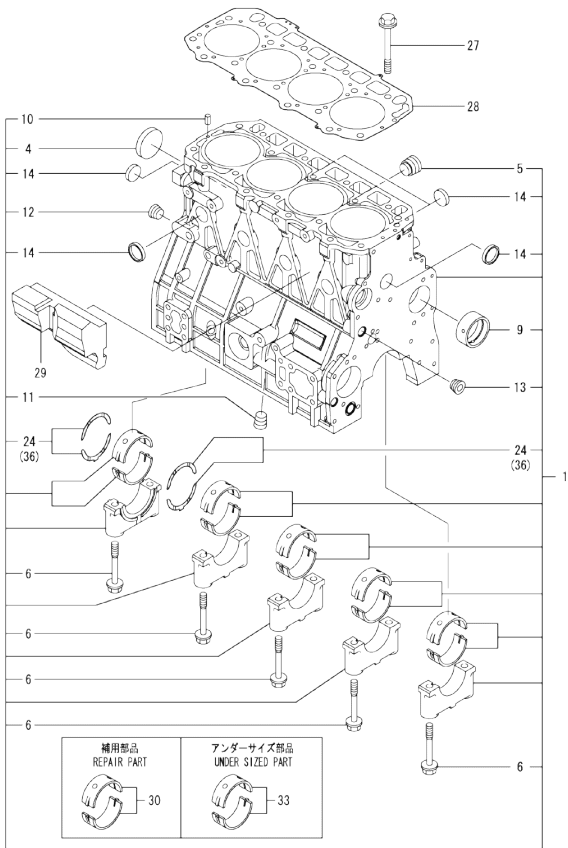
0CW10-M22100 4TNV94L-PDBWK Fig.1. CYLINDER BLOCK
