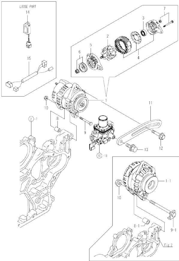
0CW10-M22100 4TNV94L-PDBWK Fig.16. GENERATOR
