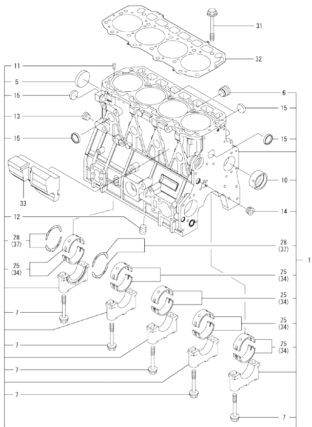
0CW10-M07400 ENGINE SECTION Fig.1. CYLINDER BLOCK
