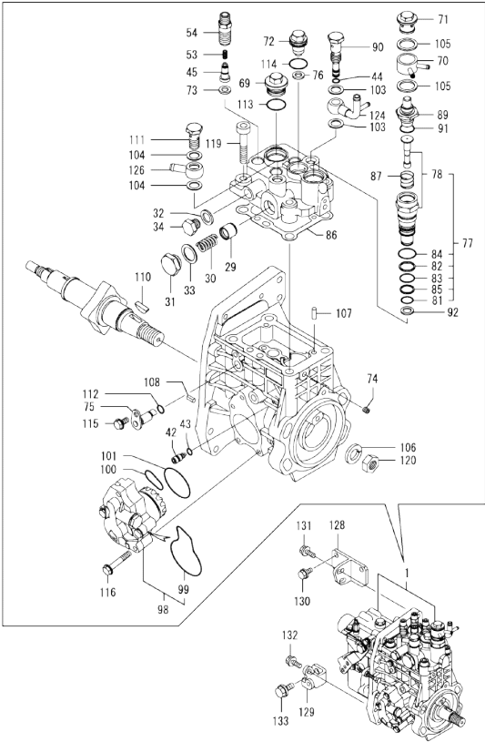
0CW10-M07400 ENGINE SECTION Fig.10. FUEL INJECTION PUMP
