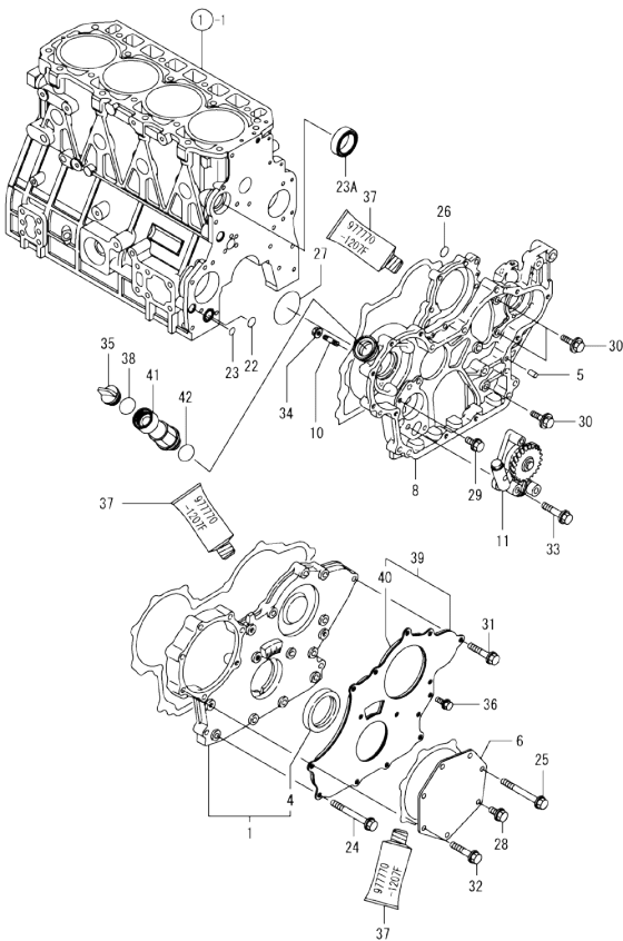
0CW10-M07400 ENGINE SECTION Fig.2. GEAR HOUSING
