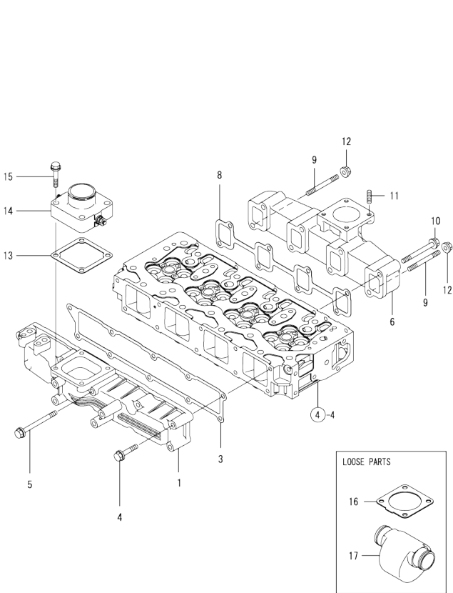
Fig.5. SUCTION & EXHAUST MANIFOLD
