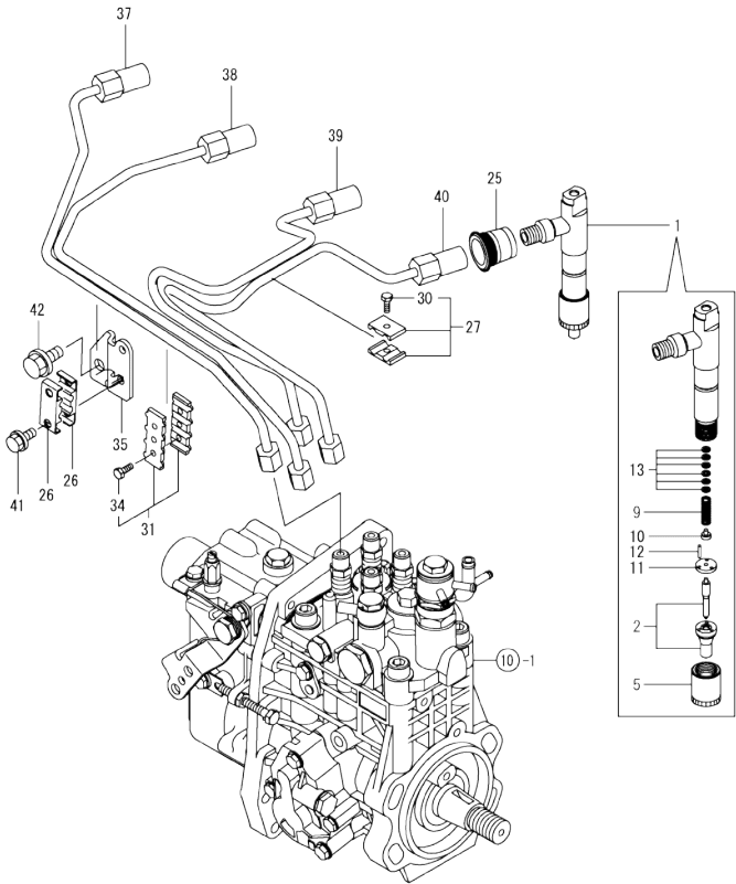
0CW10-M07400 ENGINE SECTION Fig.12. FUEL INJECTION VALVE
