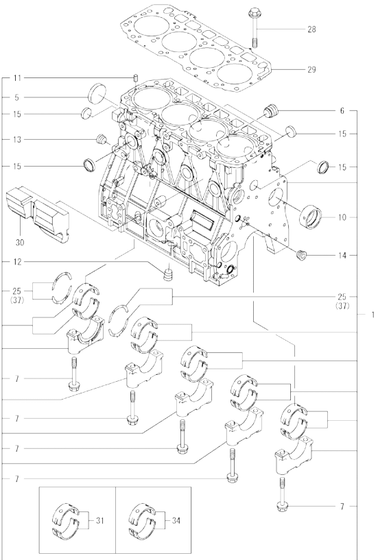
Fig.1. CYLINDER BLOCK
