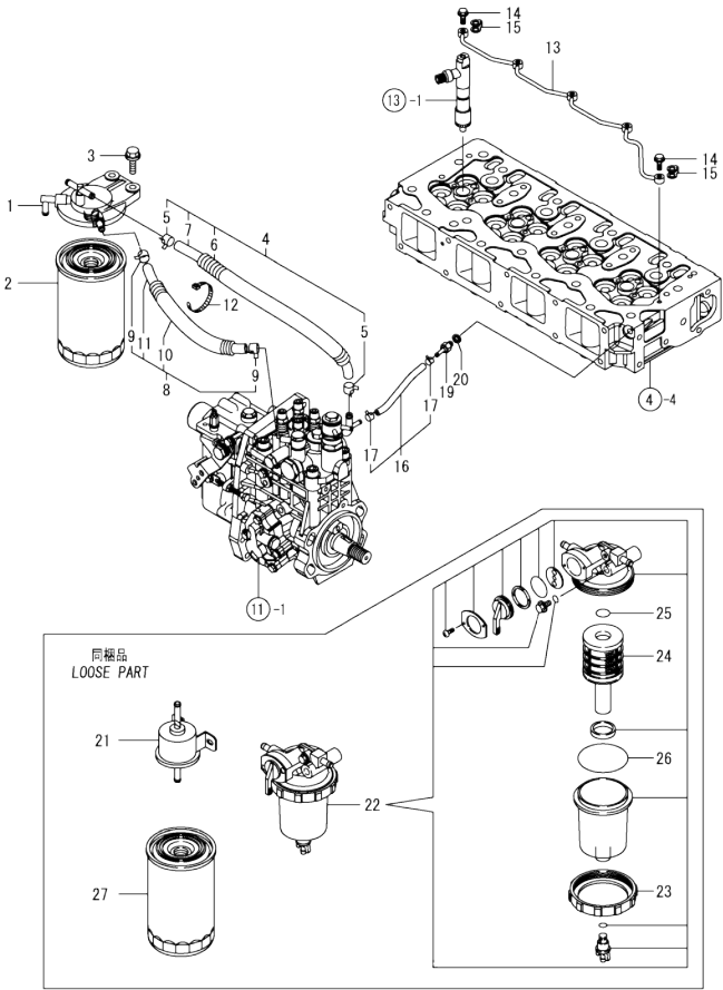
Fig.14. FUEL PIPING
