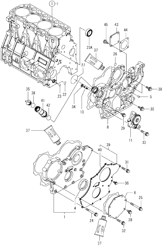
0CW10-M04901 4TNV94L-PIKA1 Fig.2. GEAR HOUSING
