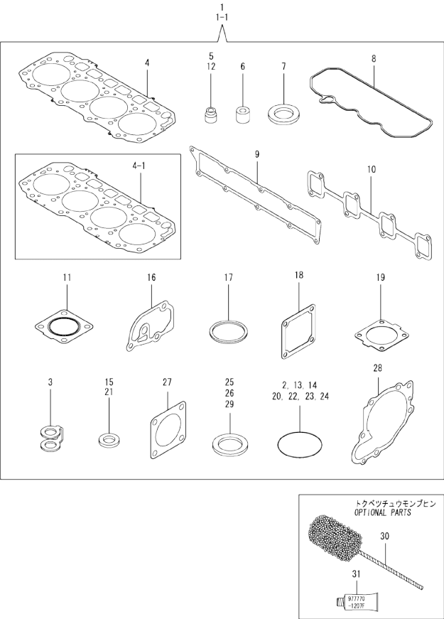
Fig.17. GASKET SET
