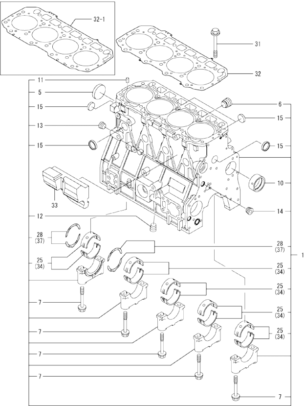
Fig.1. CYLINDER BLOCK
