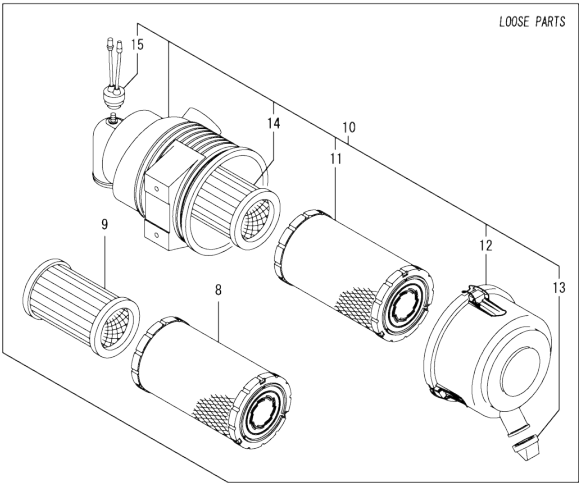
Fig.5. SUCTION MANIFOLD & AIR CLEANER
