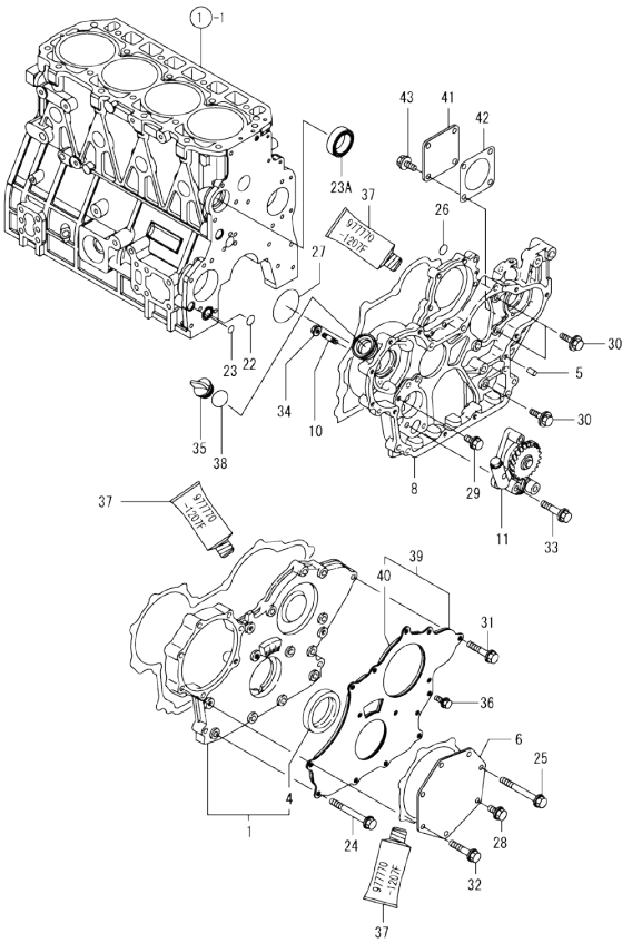
Fig.2. GEAR HOUSING
