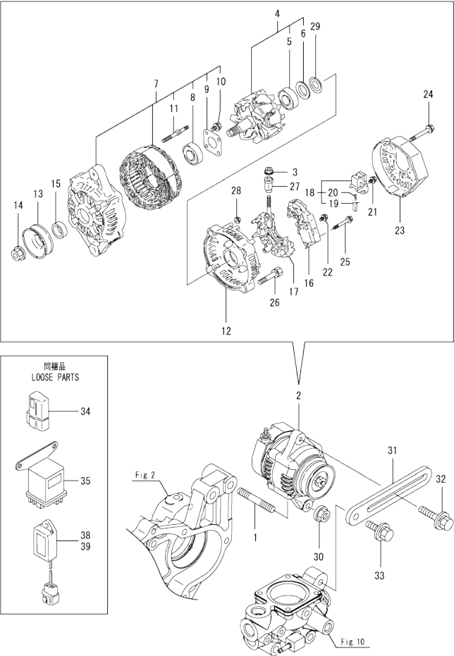
0CW10-M62900 ENGINE Fig.16. GENERATOR
