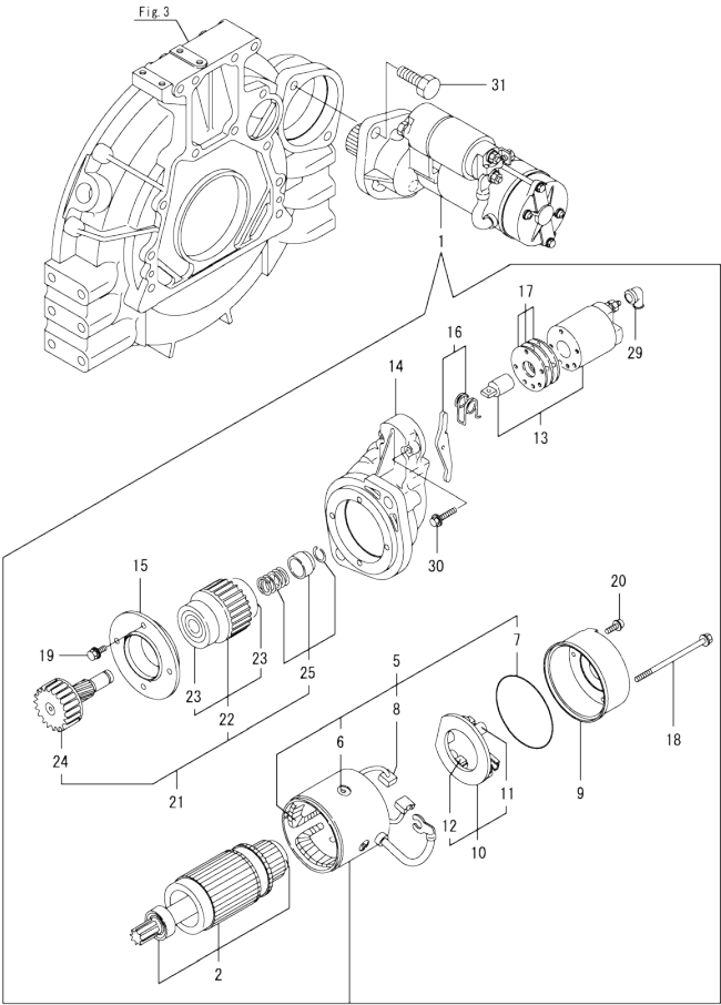
0CW10-M62900 ENGINE Fig.15. STARTING MOTOR
