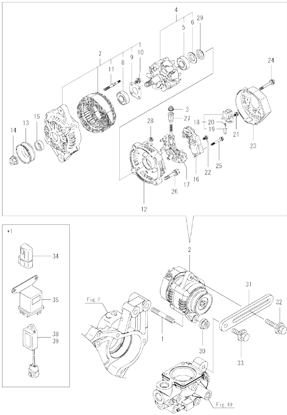
OCD50-M00600 ENGINE Fig.16. GENERATOR
