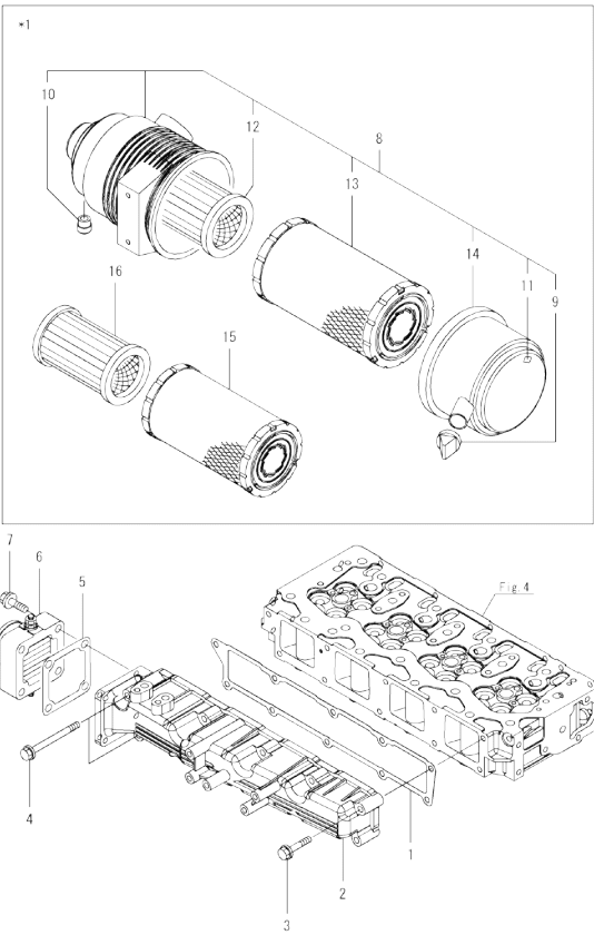
Fig.5. SUCTION MANIFOLD & AIR CLEANER
