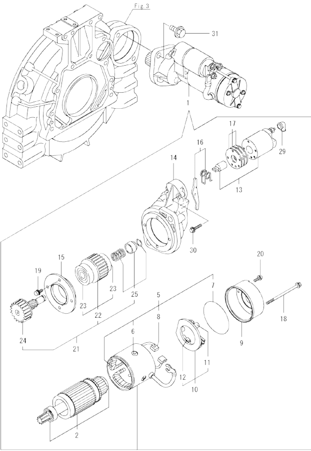
Fig.15. STARTER MOTOR
