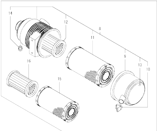
Fig.5. SUCTION MANIFOLD & AIR CLEANER
