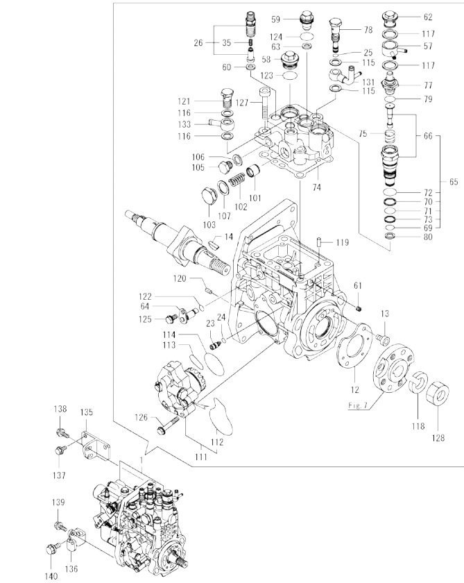
Fig.11. FUEL INJECTION PUMP
