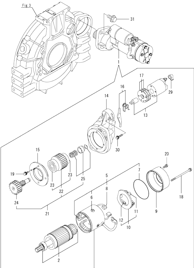
Fig.15. STARTER MOTOR
