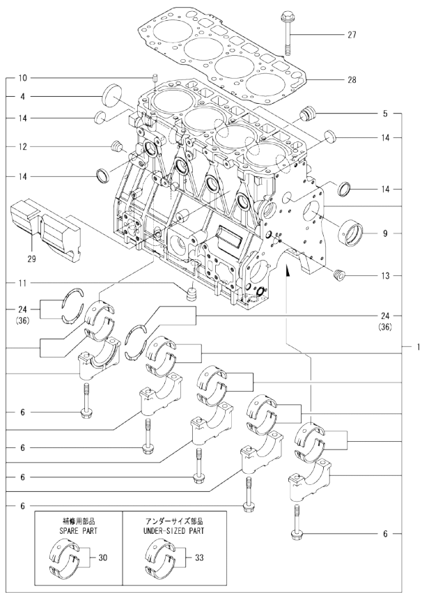
Fig.1. CYLINDER BLOCK
