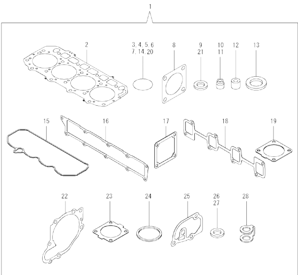
Fig.17. GASKET SET
