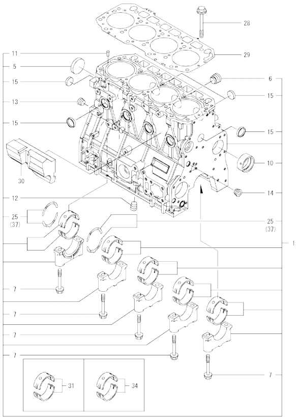
Fig.1. CYLINDER BLOCK
