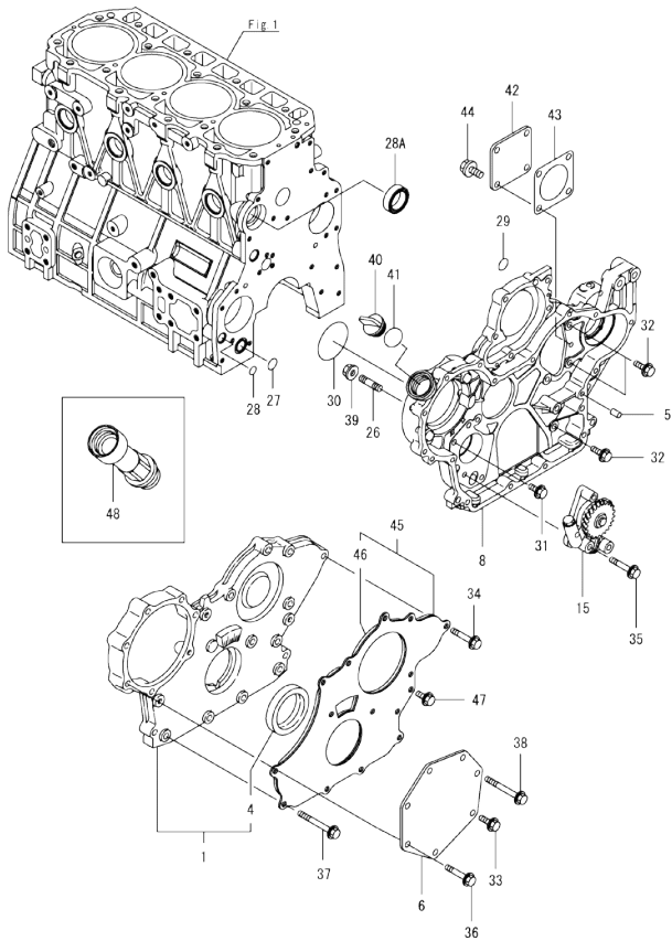
Fig.2. GEAR HOUSING
