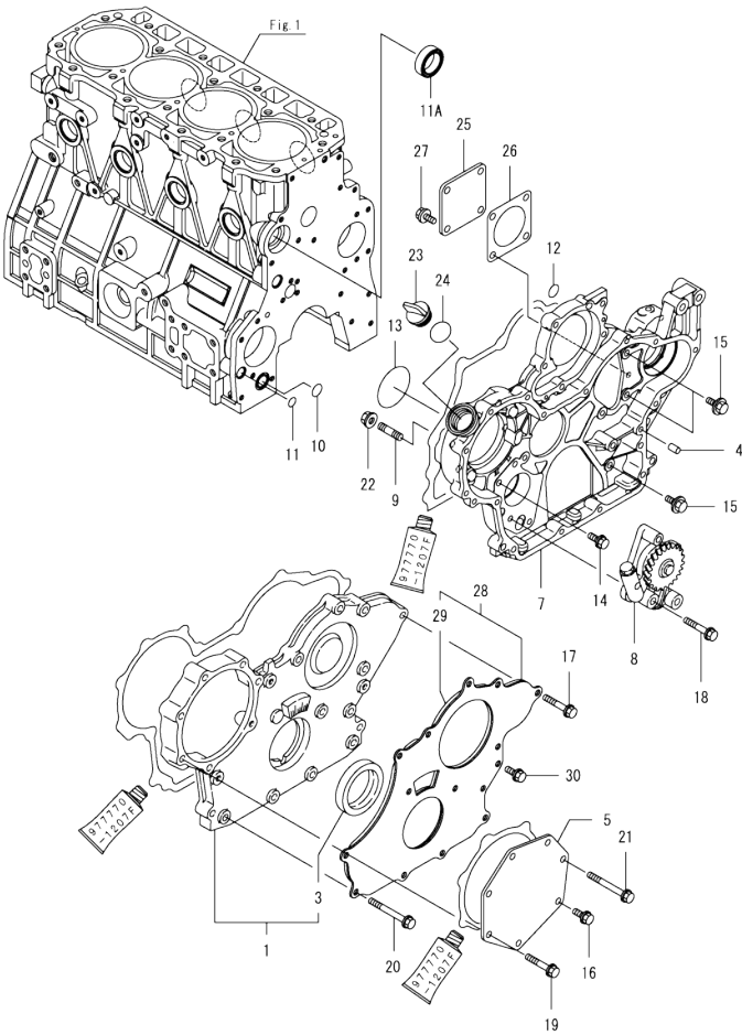
Fig.2. GEAR HOUSING
