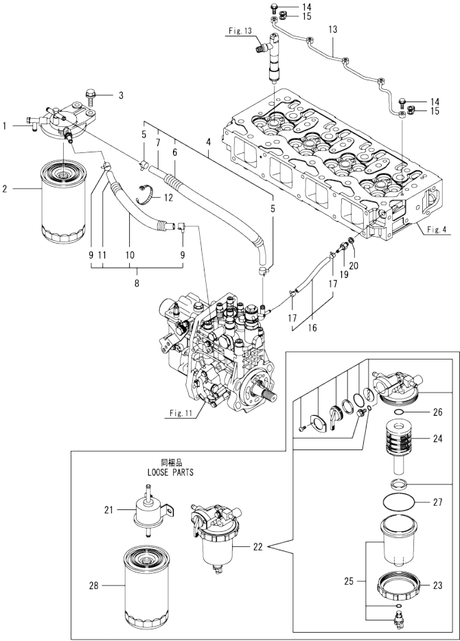
Fig.14. FUEL PIPING
