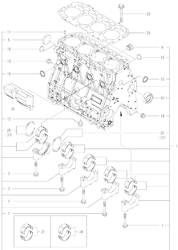
Fig.1. CYLINDER BLOCK
