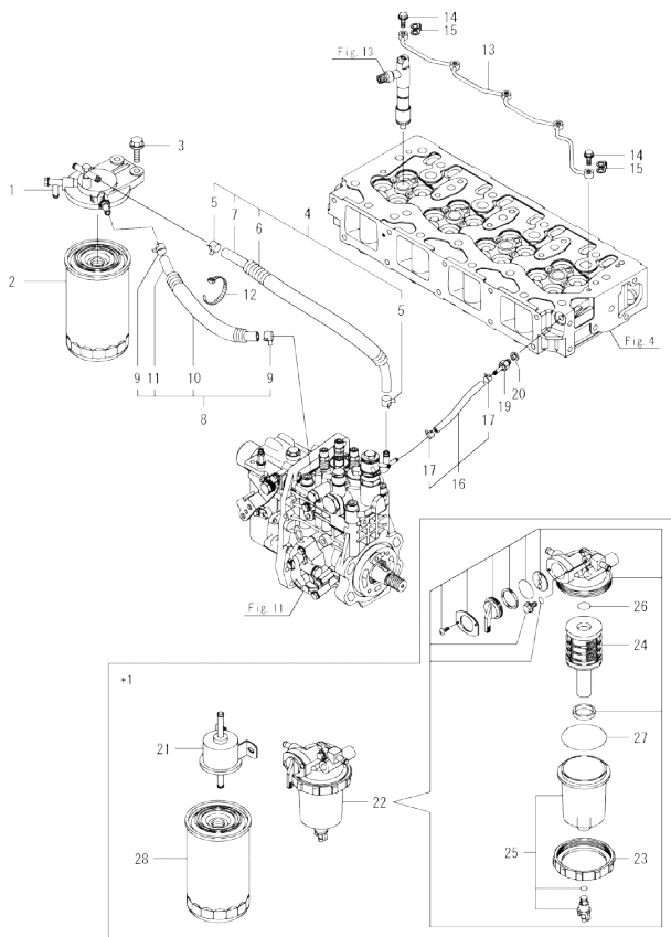
Fig.14. FUEL PIPING
