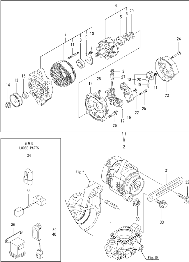
0CW10-M74400 ENGINE Fig.16. GENERATOR
