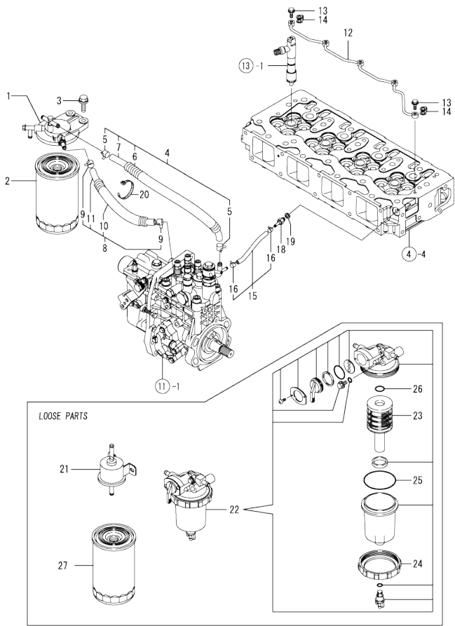
Fig.14. FUEL LINE
