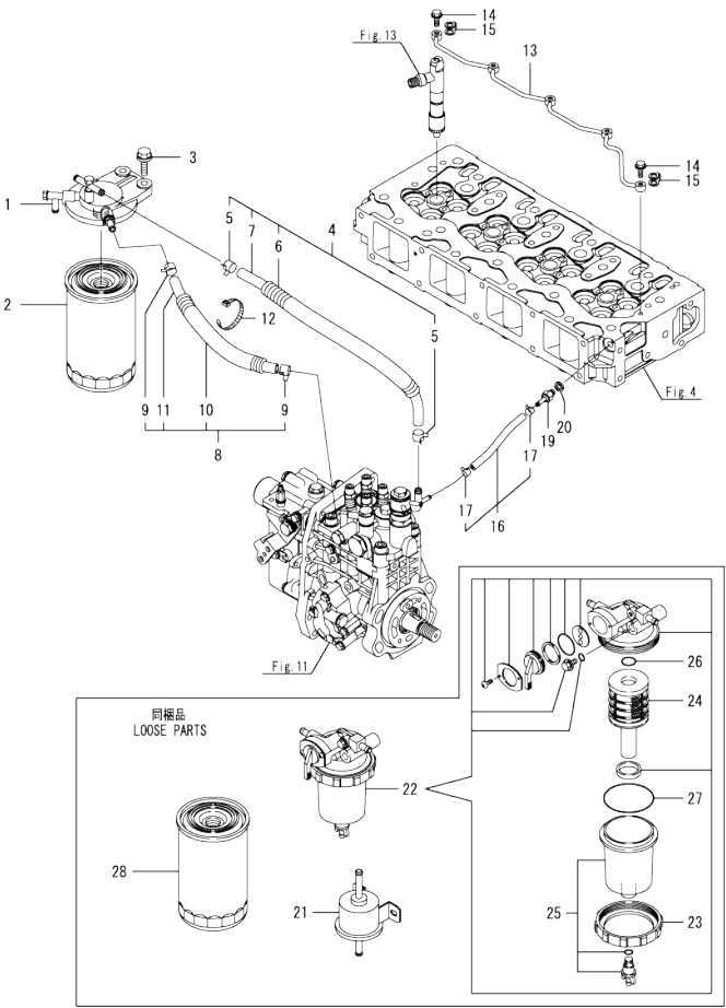
Fig.14. FUEL PIPING
