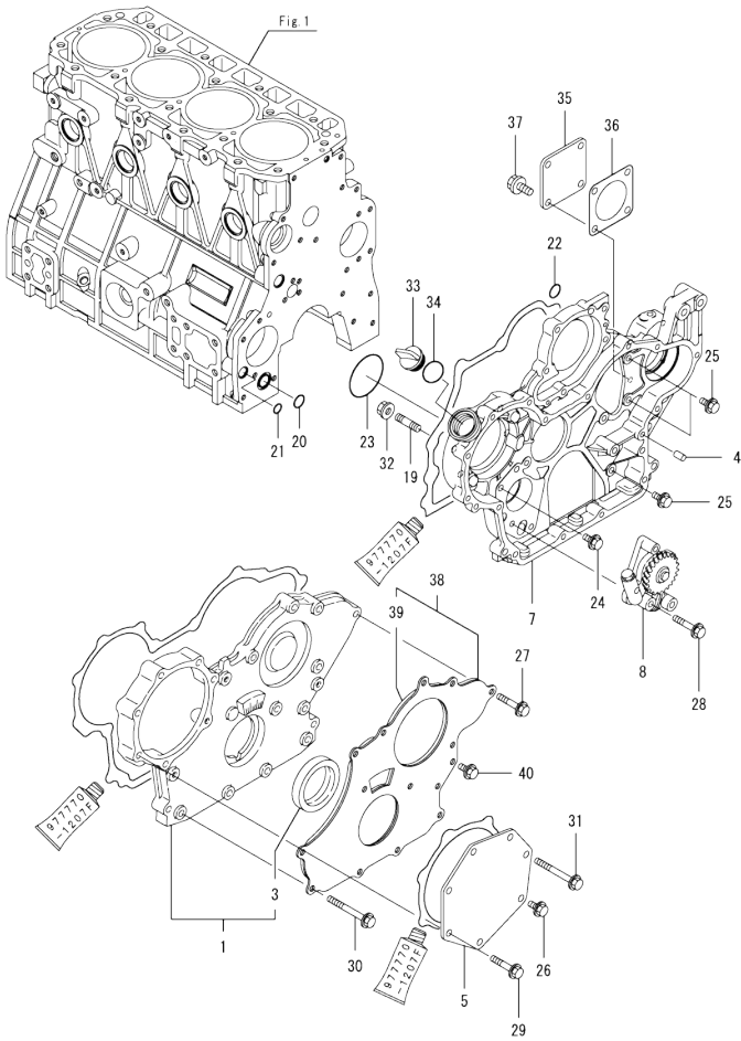
Fig.2. GEAR HOUSING
