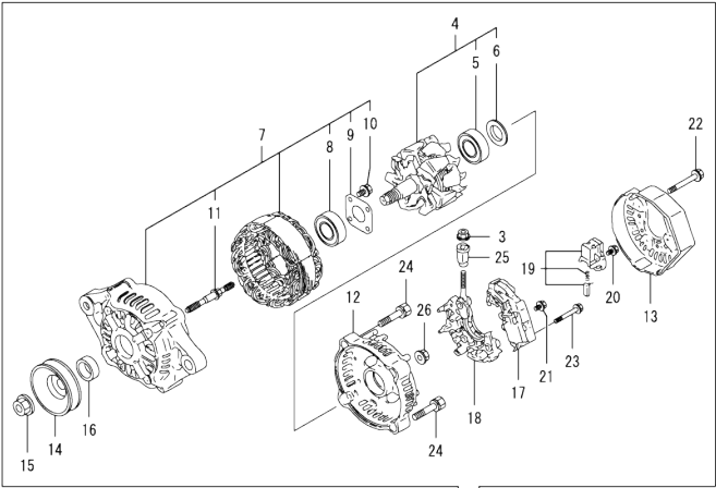
0CW10-M74300 ENGINE Fig.16. GENERATOR
