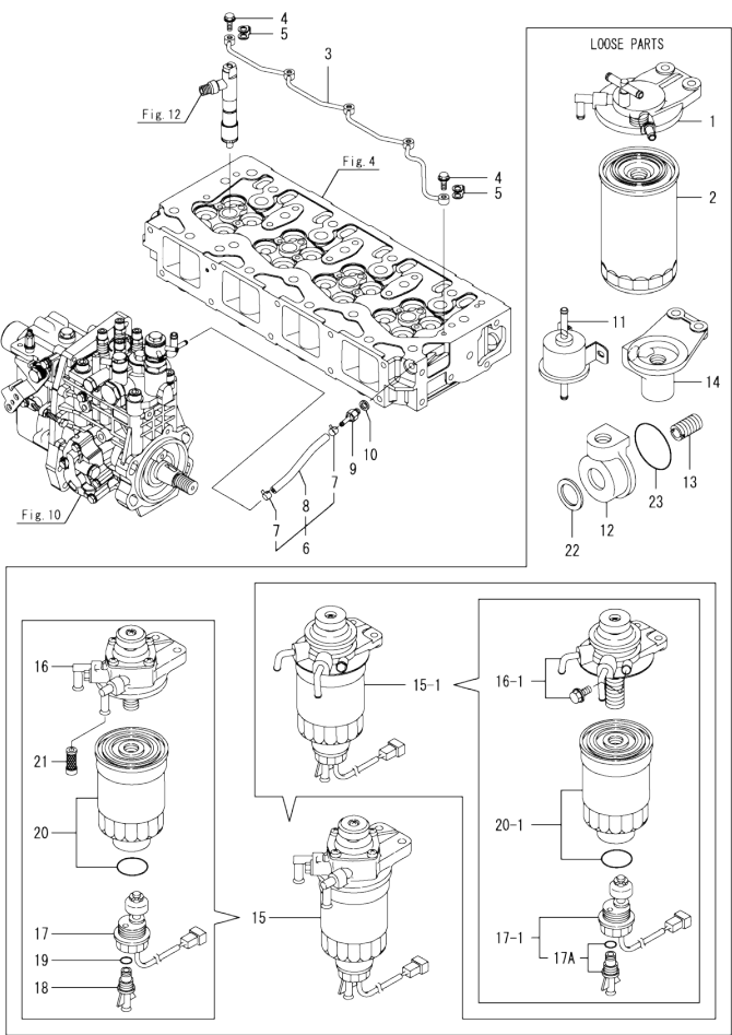
Fig.13. FUEL PIPE
