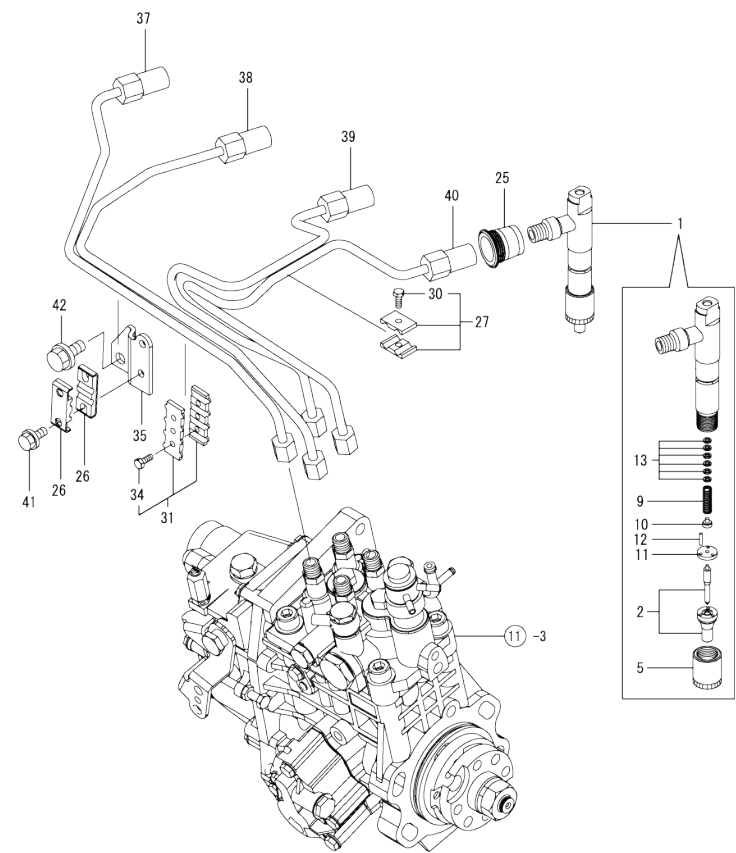
Fig.12. FUEL INJECTION VALVE
