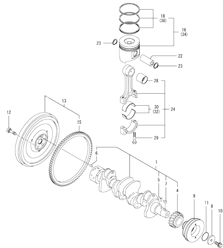
Fig.8. CRANKSHAFT & PISTON
