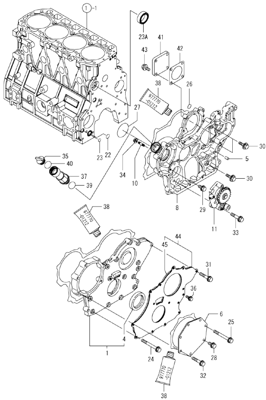
OCV10-M89100 4TNV94L-XDB Fig.2. GEAR HOUSING
