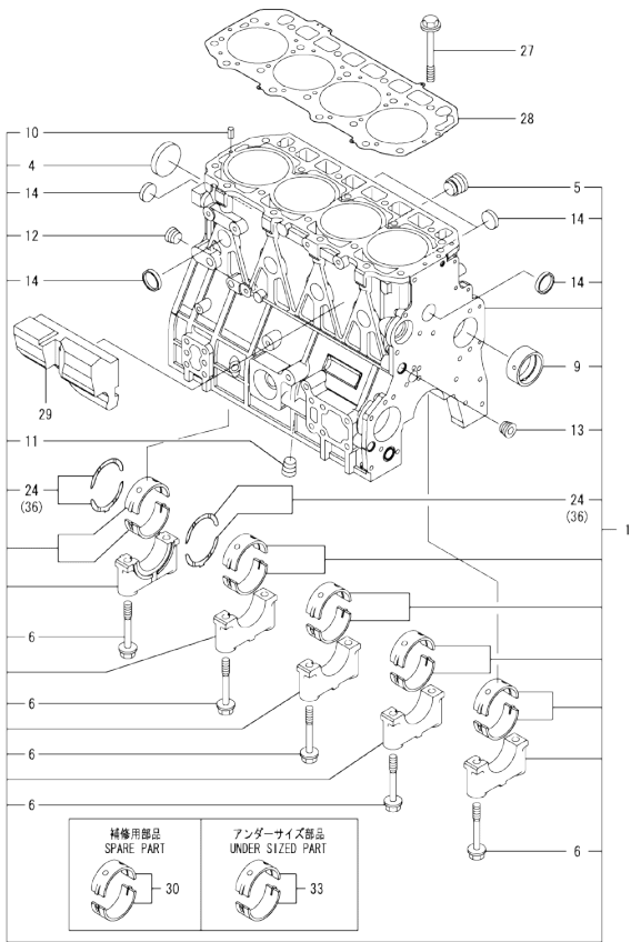
0CW10-M22001 4TNV94L-XDBKC Fig.1. CYLINDER BLOCK
