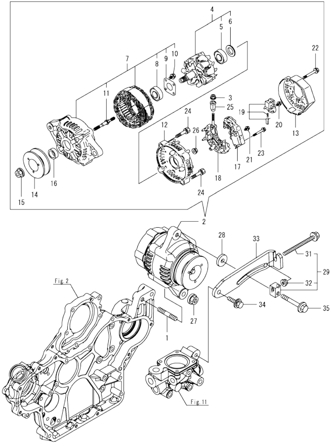
OCD50-M06360 ENGINE Fig.16. GENERATOR
