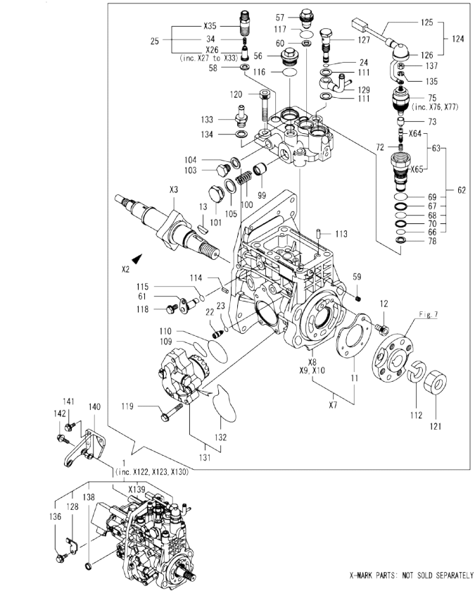
Fig.11. FUEL INJECTION PUMP
