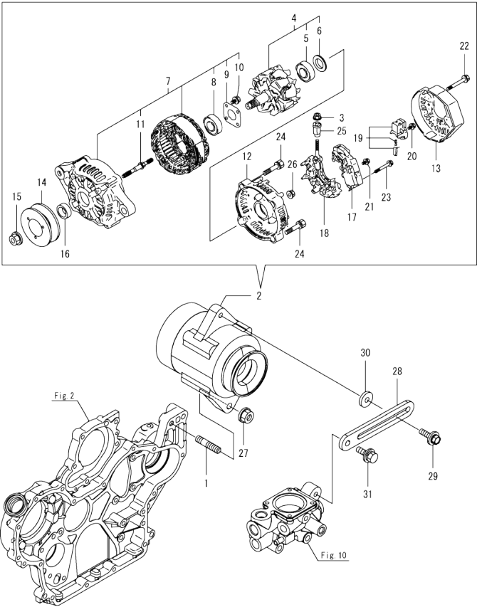
OCD50-M04040 ENGINE Fig.16. GENERATOR
