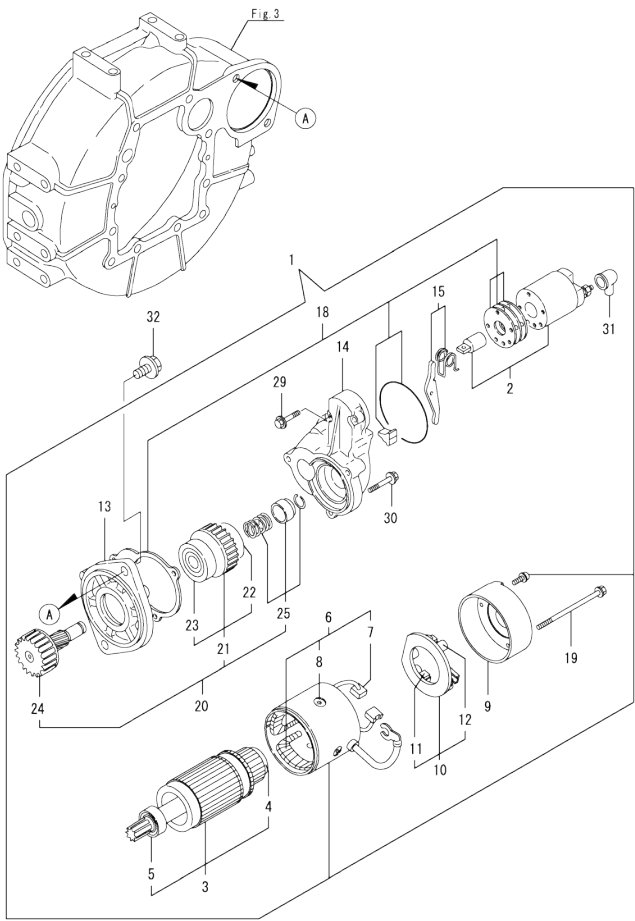
Fig.15. STARTING MOTOR
