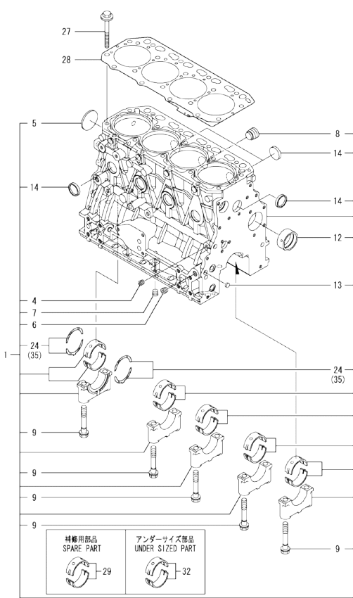
Fig.1. CYLINDER BLOCK
