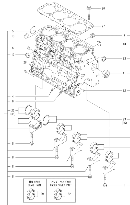
Fig.1. CYLINDER BLOCK
