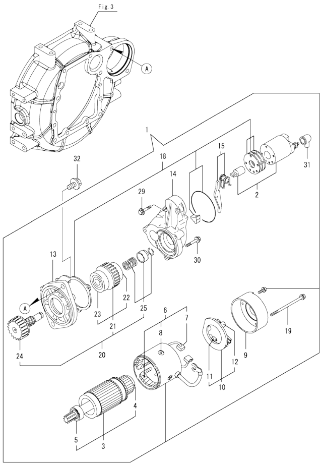
Fig.15. STARTER MOTOR
