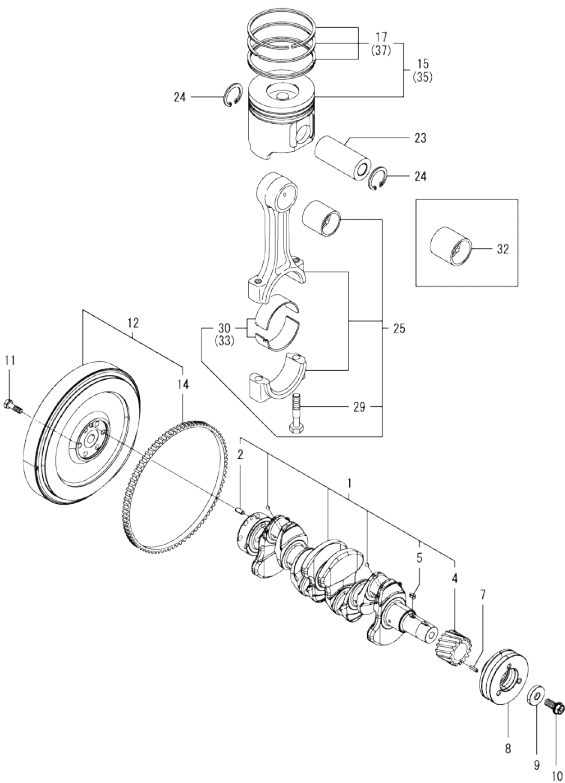
Fig.8. CRANKSHAFT & PISTON
