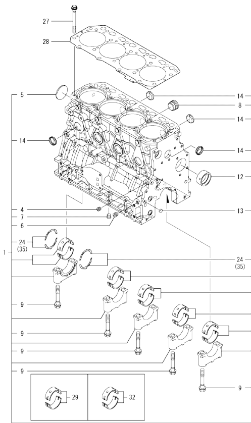
Fig.1. CYLINDER BLOCK
