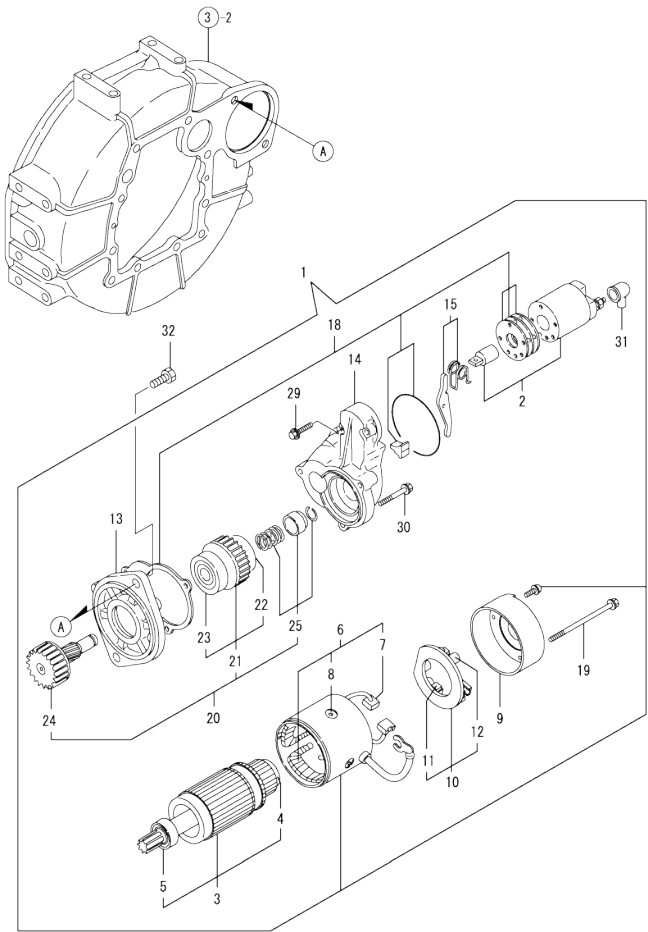
Fig.15. STARTING MOTOR
