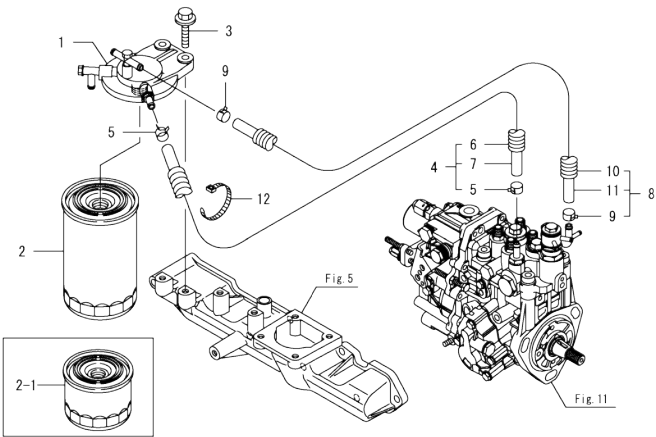
Fig.14. FUEL PIPE
