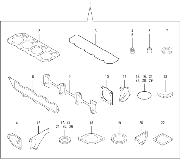
Fig.17. GASKET SET
