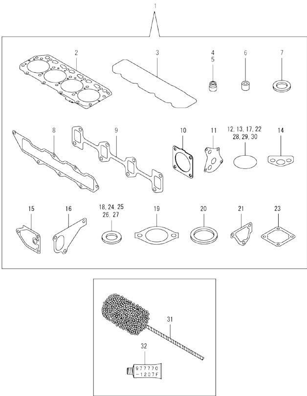
Fig.17. GASKET SET
