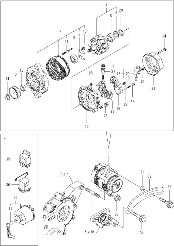
OCD11-M19300 ENGINE Fig.16. GENERATOR
