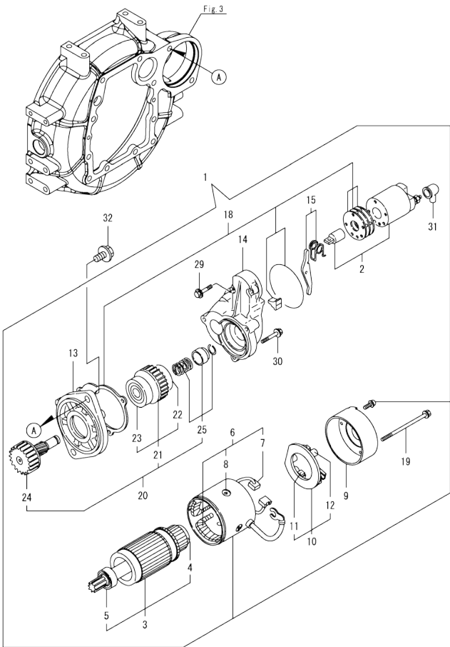
Fig.18. (15A)STARTER MOTOR(FROM ES9364)
