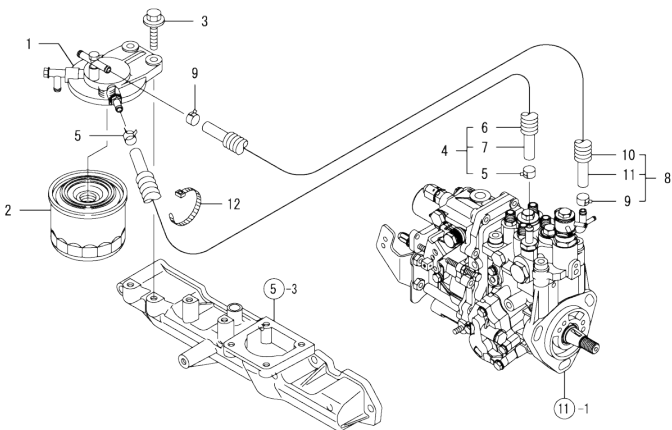
Fig.14. FUEL LINE
