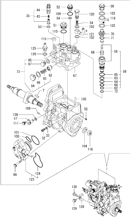
Fig.11. FUEL INJECTION PUMP
