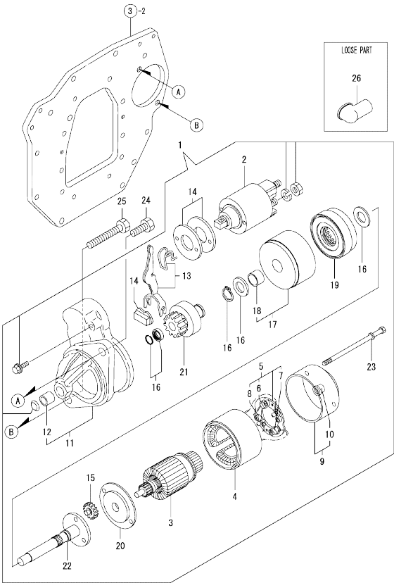
0CW10-M43300 3TNV88-BDCR Fig.15. STARTING MOTOR
