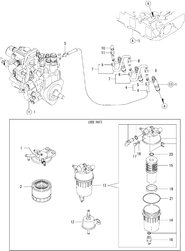
Fig.14. FUEL LINE
