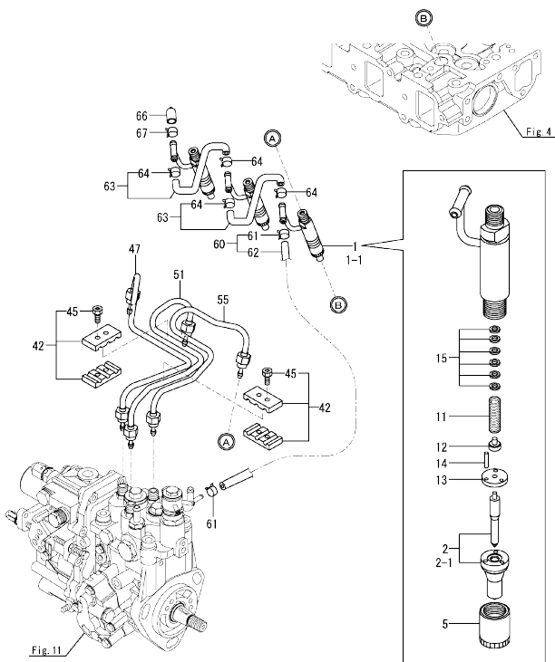
Fig.13. FUEL INJECTION VALVE
