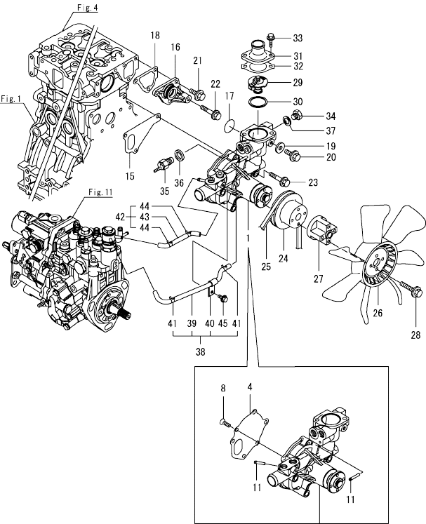
Fig.10. COOLING WATER SYSTEM
