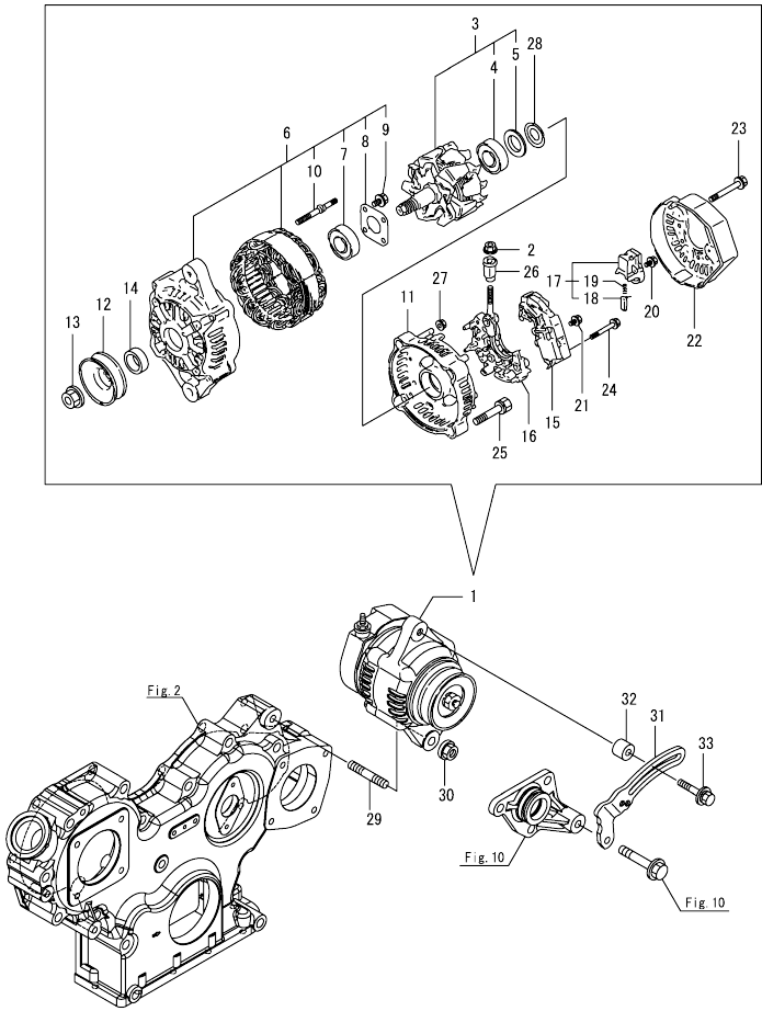
OCD50-M05600 ENGINE Fig.16. GENERATOR
