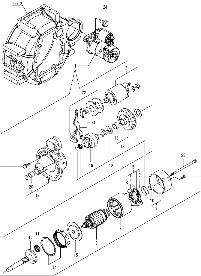
Fig.15. STARTER MOTOR
