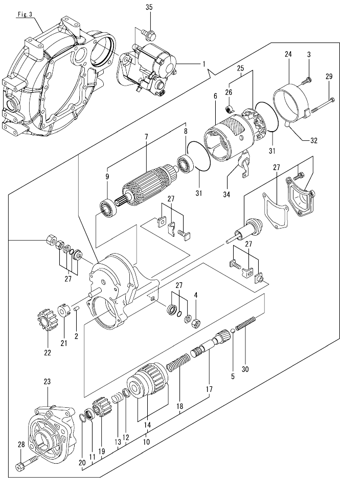
Fig.15. STARTER MOTOR
