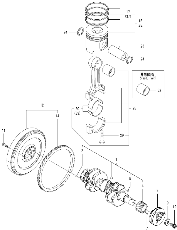
Fig.8. CRANKSHAFT & PISTON
