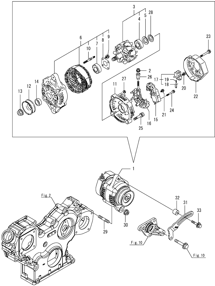
OCD50-M03650 ENGINE Fig.16. GENERATOR
