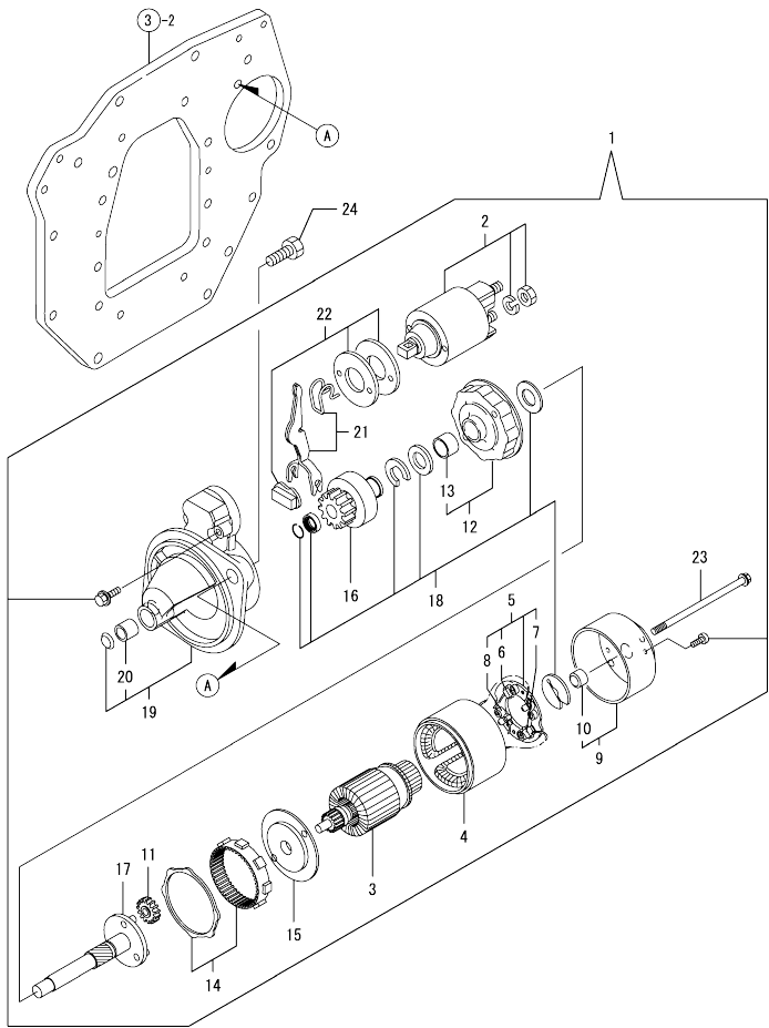
Fig.15. STARTING MOTOR
