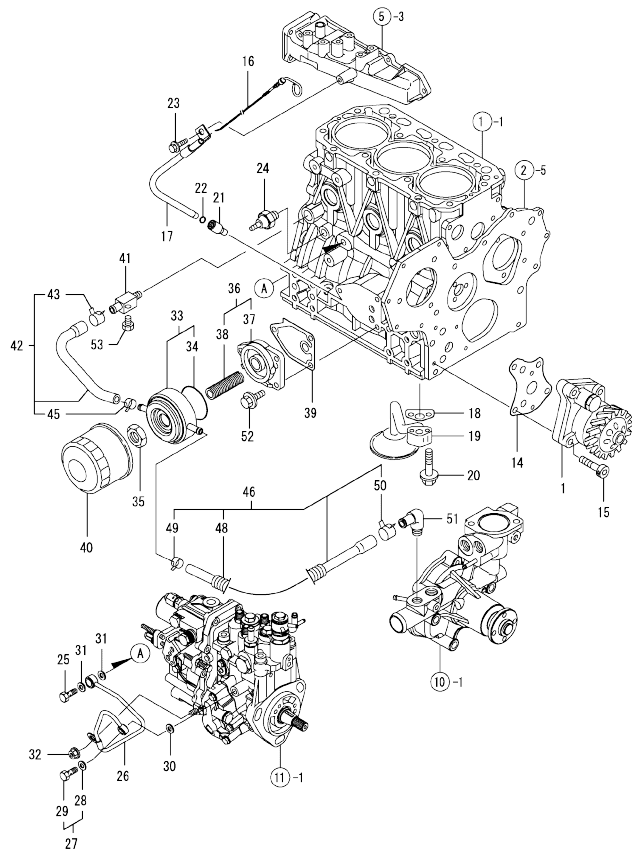
Fig.9. LUB.OIL SYSTEM
