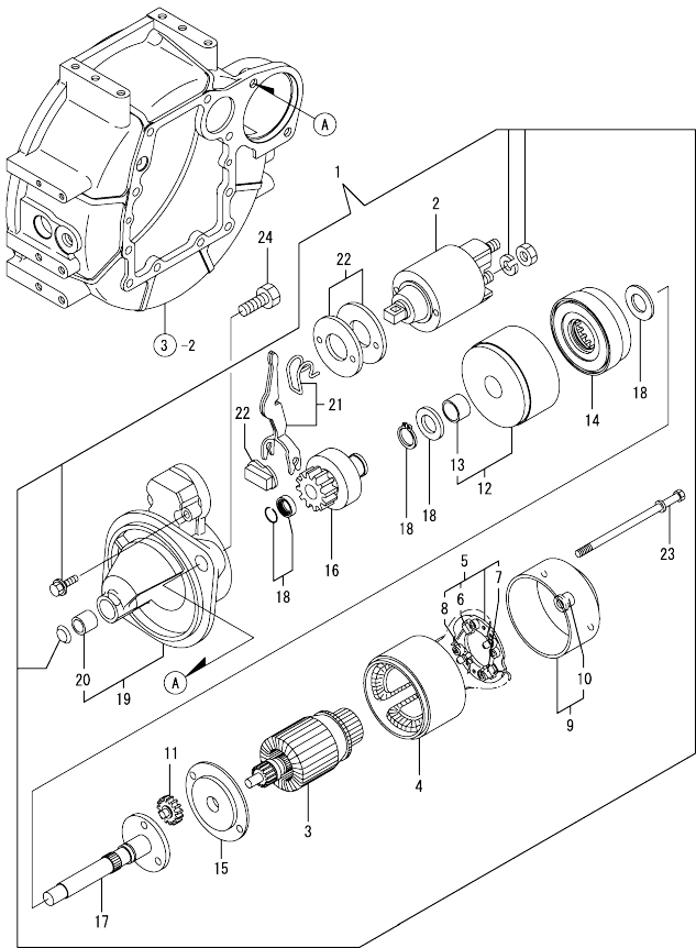
0CW10-M43800 3TNV88-BDSA Fig.15. STARTING MOTOR
