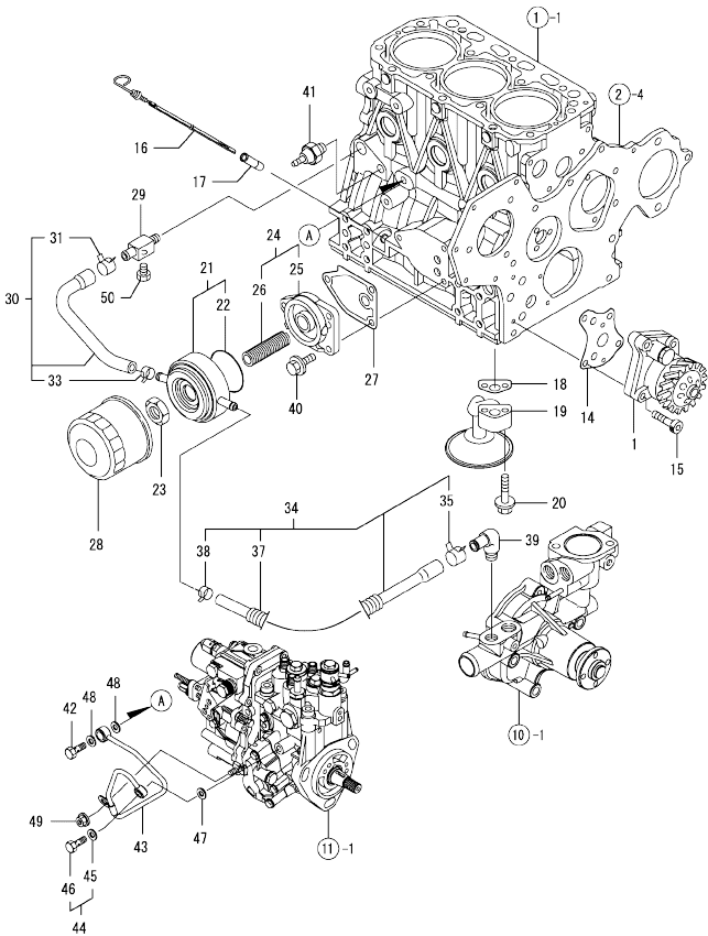
0CW10-M43800 3TNV88-BDSA Fig.9. LUB.OIL SYSTEM
