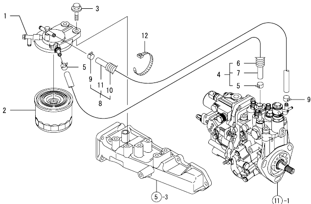
Fig.14. FUEL LINE
