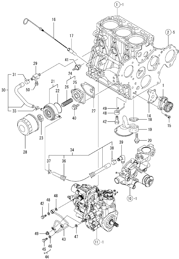
0CW10-M23200 3TNV88-BDSA2 Fig.9. LUB.OIL SYSTEM
