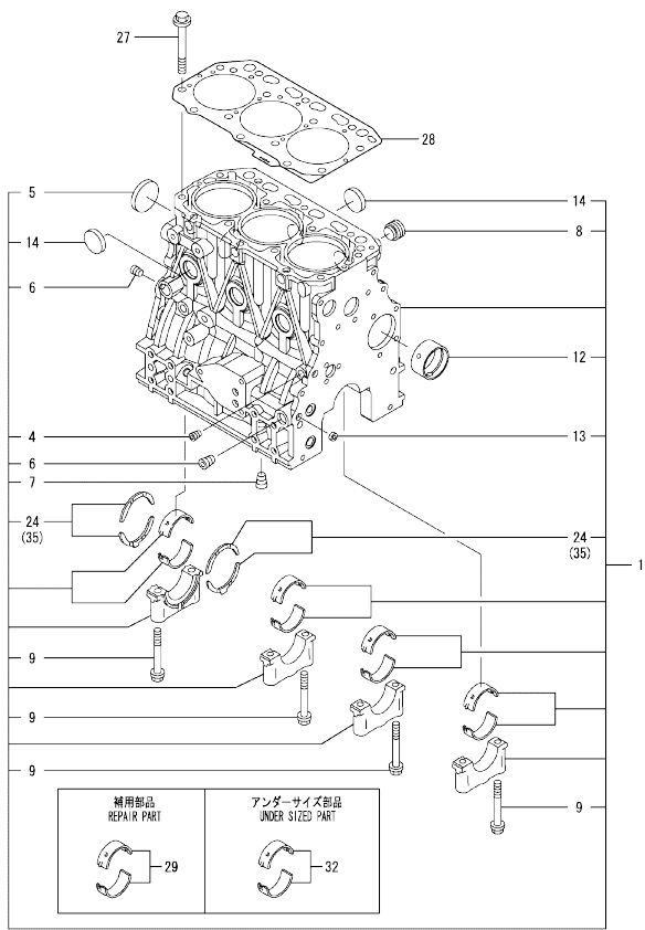
0CW10-M23200 3TNV88-BDSA2 Fig.1. CYLINDER BLOCK
