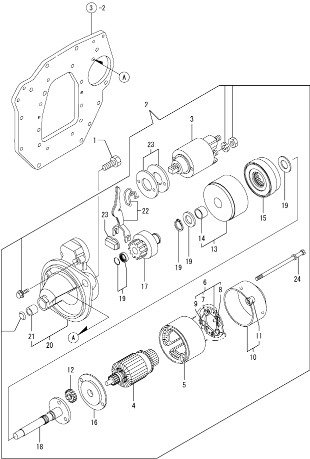
0CW10-M23300 3TNV88-BDSA3 Fig.15. STARTING MOTOR
