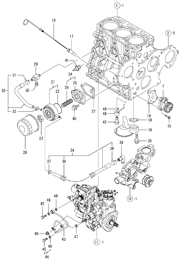
0CW10-M23300 3TNV88-BDSA3 Fig.9. LUB.OIL SYSTEM
