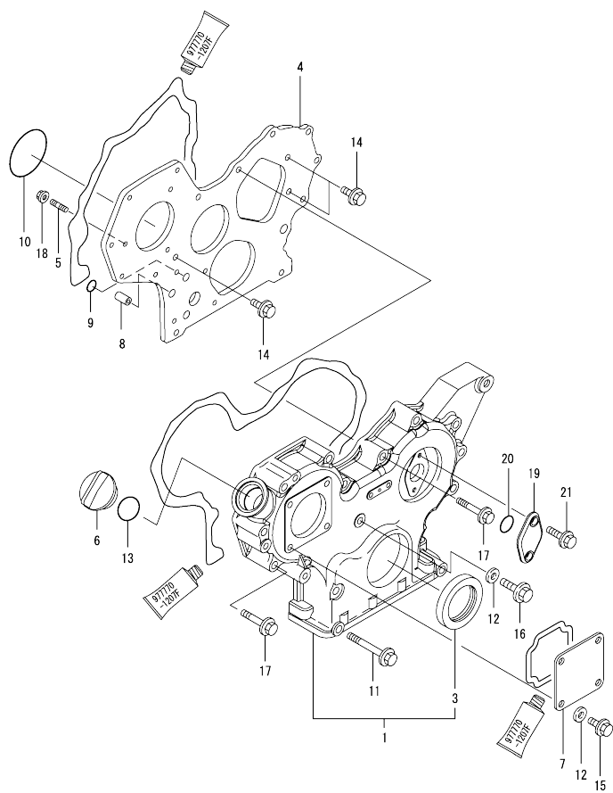
Fig.2. GEAR HOUSING
