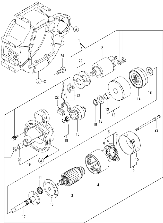
Fig.15. STARTING MOTOR
