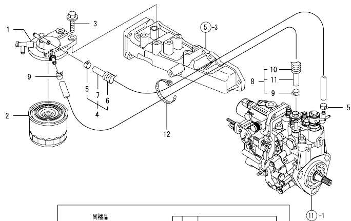
Fig.14. FUEL LINE
