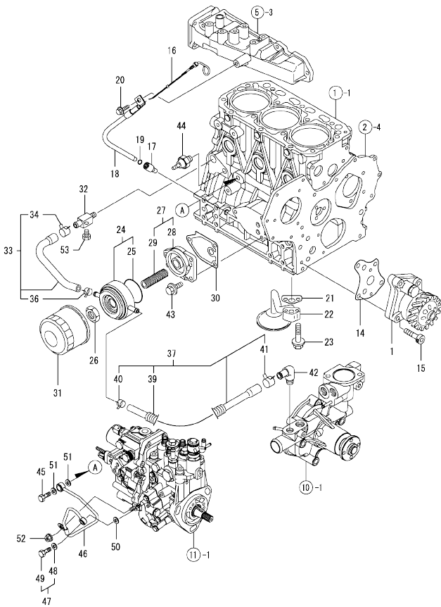
Fig.9. LUB.OIL SYSTEM
