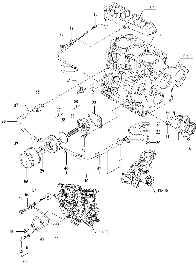
Fig.9. LUB.OIL SYSTEM
