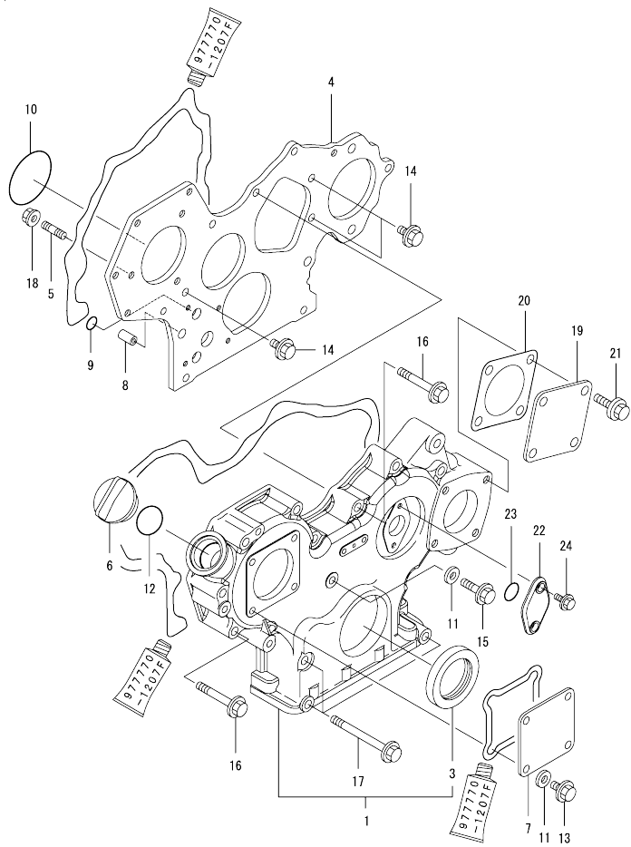
Fig.2. GEAR HOUSING
