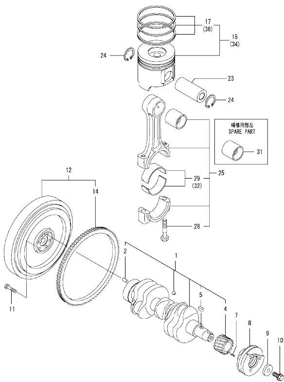
Fig.8. CRANKSHAFT & PISTON
