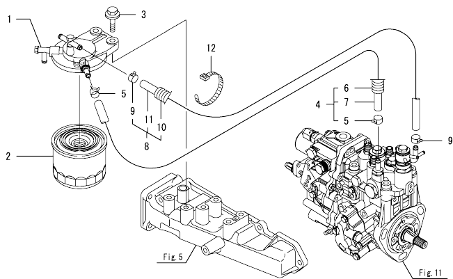
Fig.14. FUEL LINE
