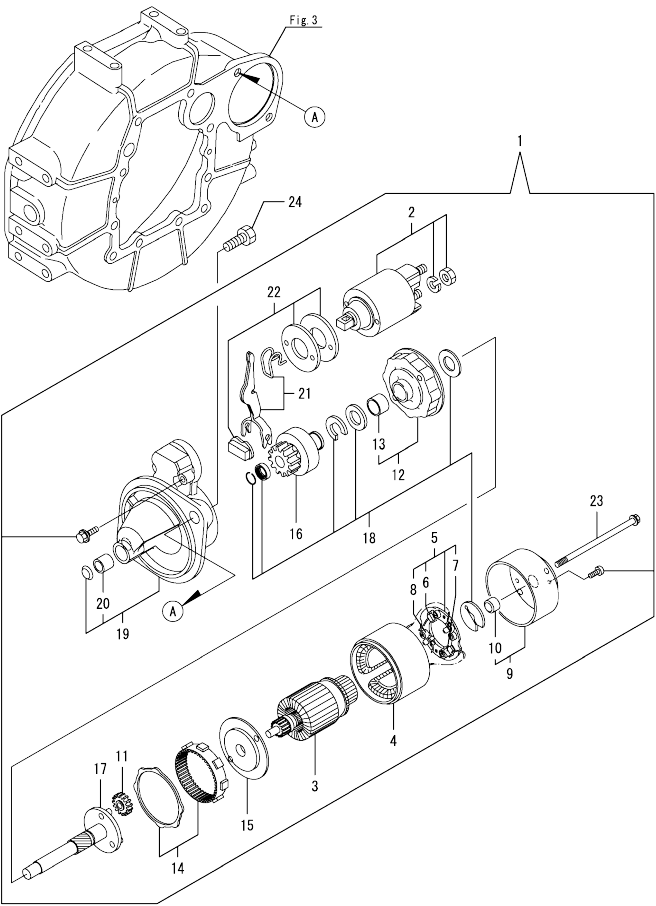
Fig.15. STARTER MOTOR
