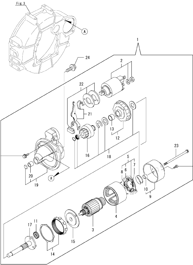
Fig.15. STARTER MOTOR
