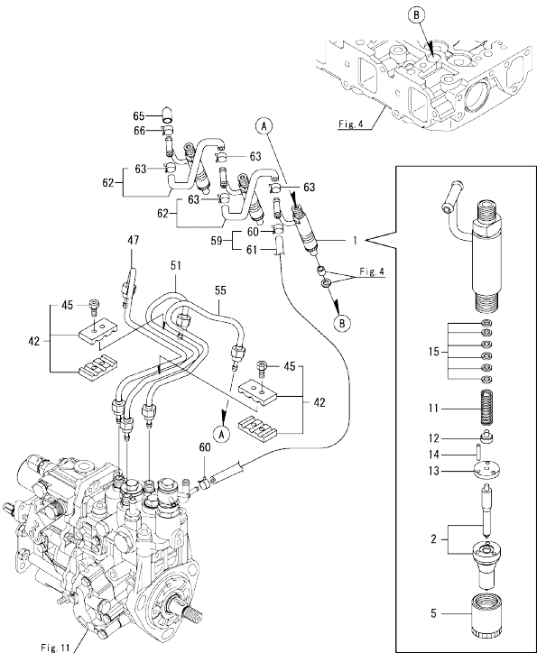
Fig.13. FUEL INJECTION VALVE
