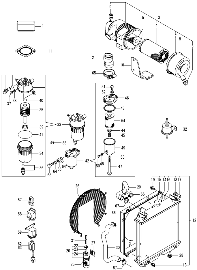
OCD50-M02940 ENGINE Fig.17. ACCESSORY
