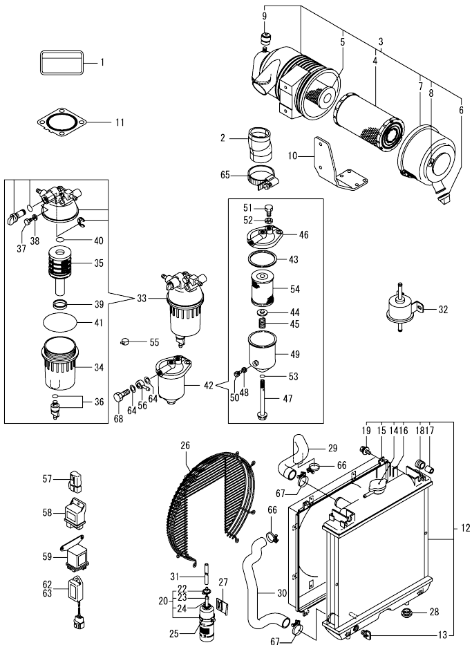
Fig.17. ACCESSORY
