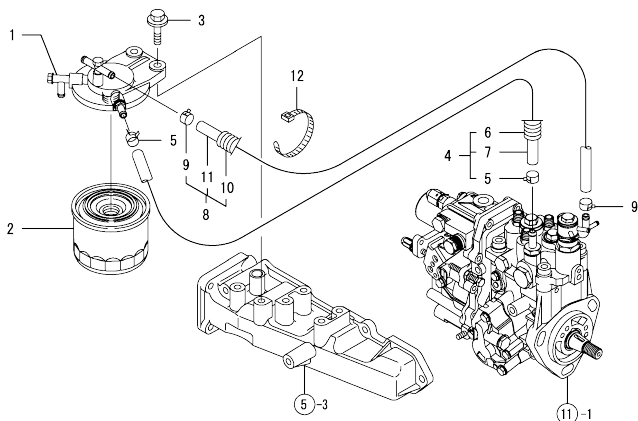
Fig.14. FUEL PIPE
