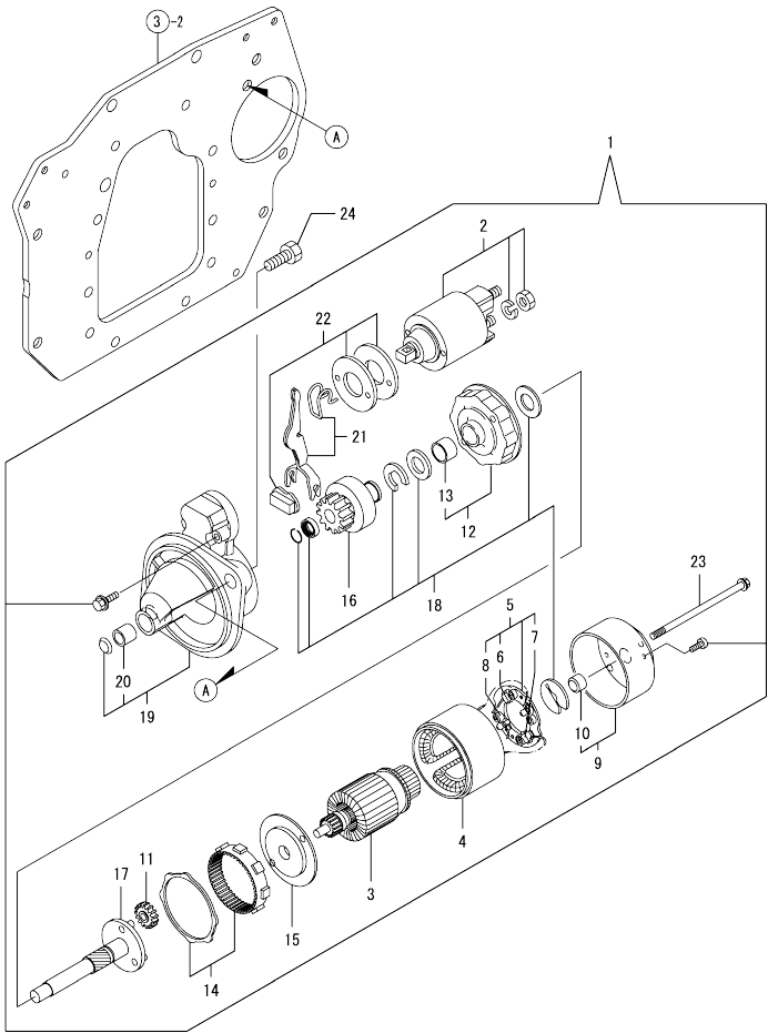
Fig.15. STARTER MOTOR
