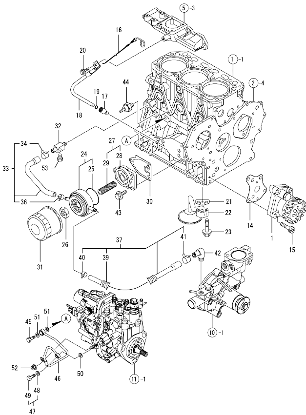
Fig.9. LUB.OIL SYSTEM
