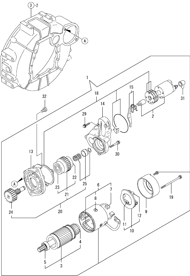
0CW10-M35800 3TNV88-BDWL Fig.15. STARTING MOTOR
