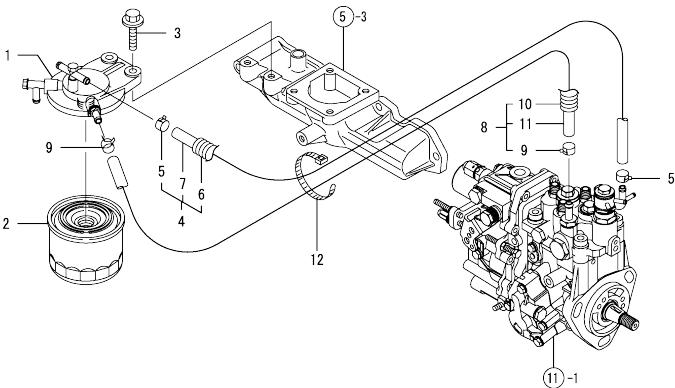
Fig.14. FUEL LINE
