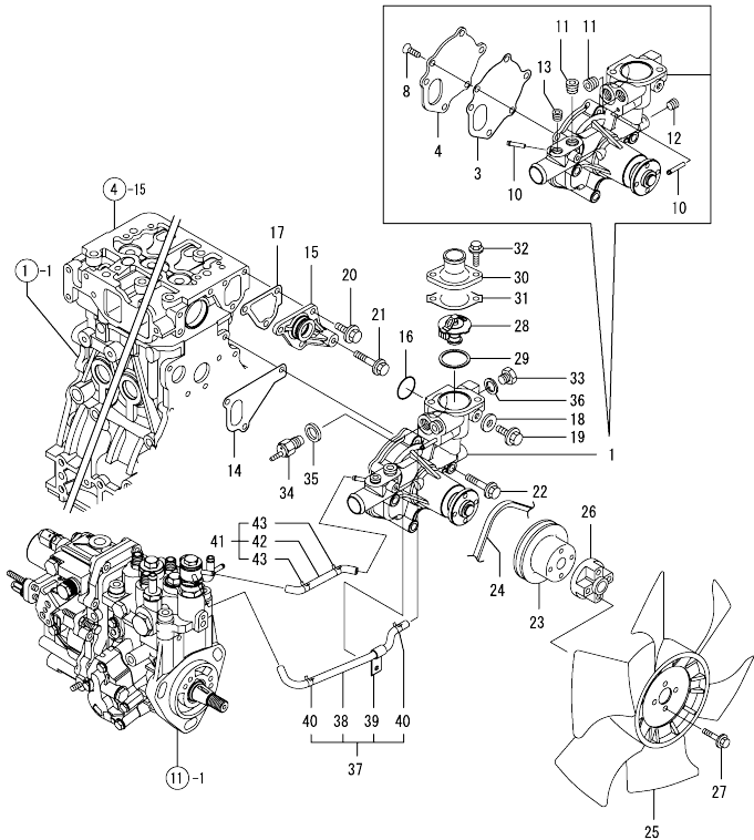
Fig.10. COOLING WATER SYSTEM
