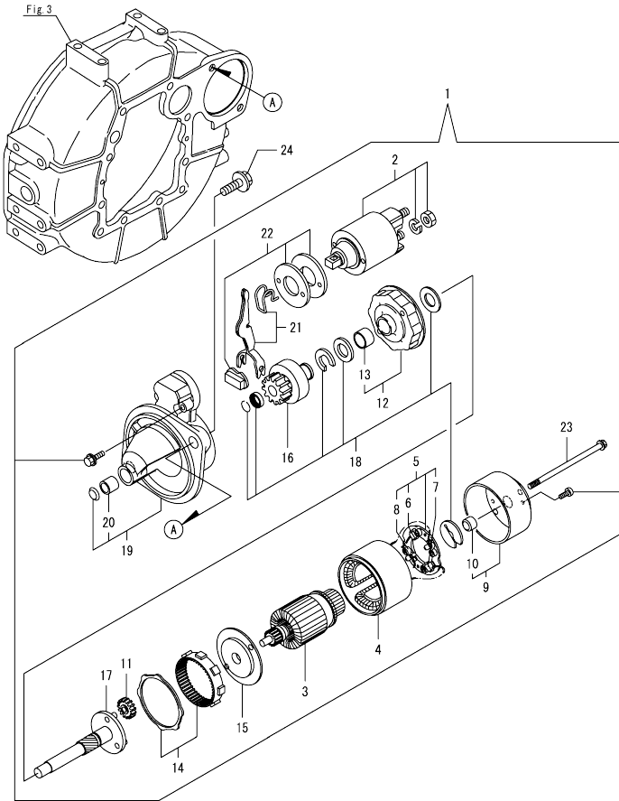
Fig.15. STARTER MOTOR
